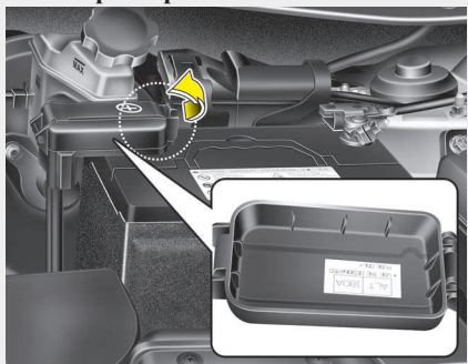
Fusible principal
